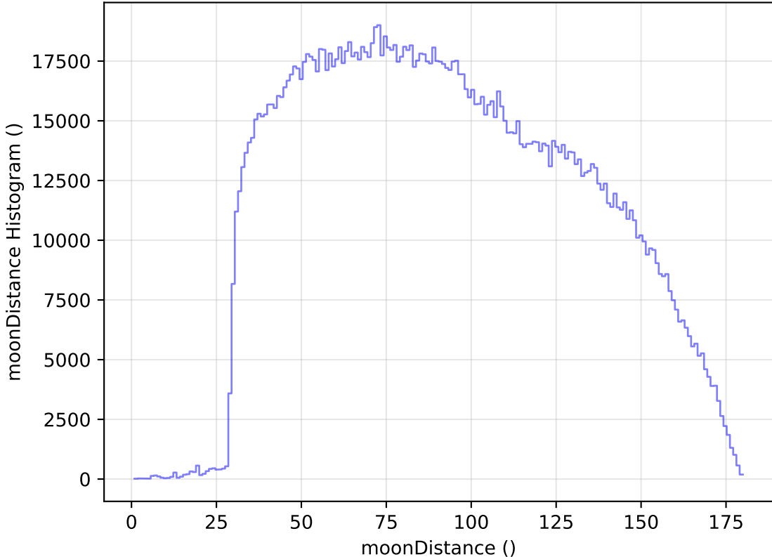
too_elab_heavy_r32_d2_ugrizy_v3.4_10yrs All sky all bands: moonDistance Histogram
