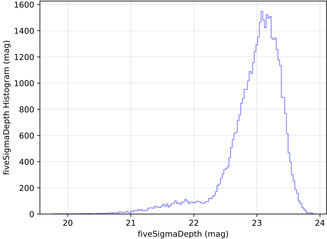
too_elab_heavy_r32_d2_ugrizy_v3.4_10yrs Yr 1 z band: fiveSigmaDepth Histogram
