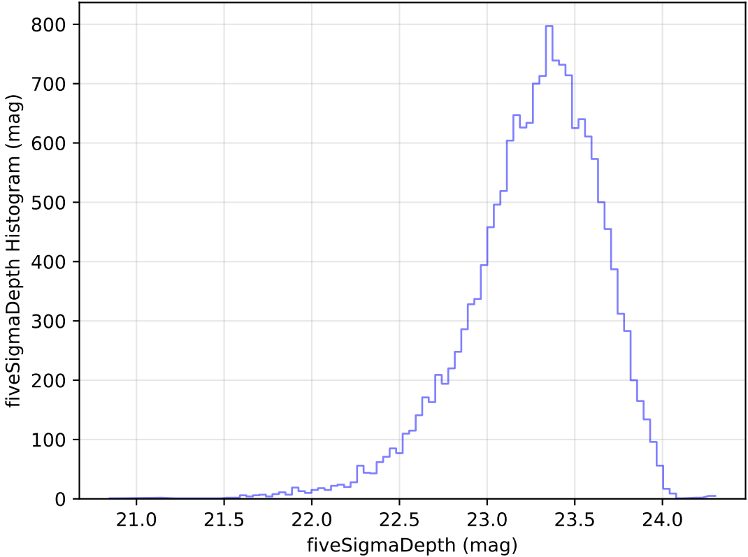
too_elab_heavy_r32_d2_ugrizy_v3.4_10yrs Yr 1 u band: fiveSigmaDepth Histogram
