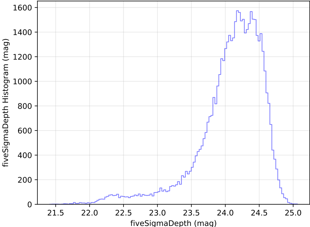
too_elab_heavy_r32_d2_ugrizy_v3.4_10yrs Yr 1 r band: fiveSigmaDepth Histogram
