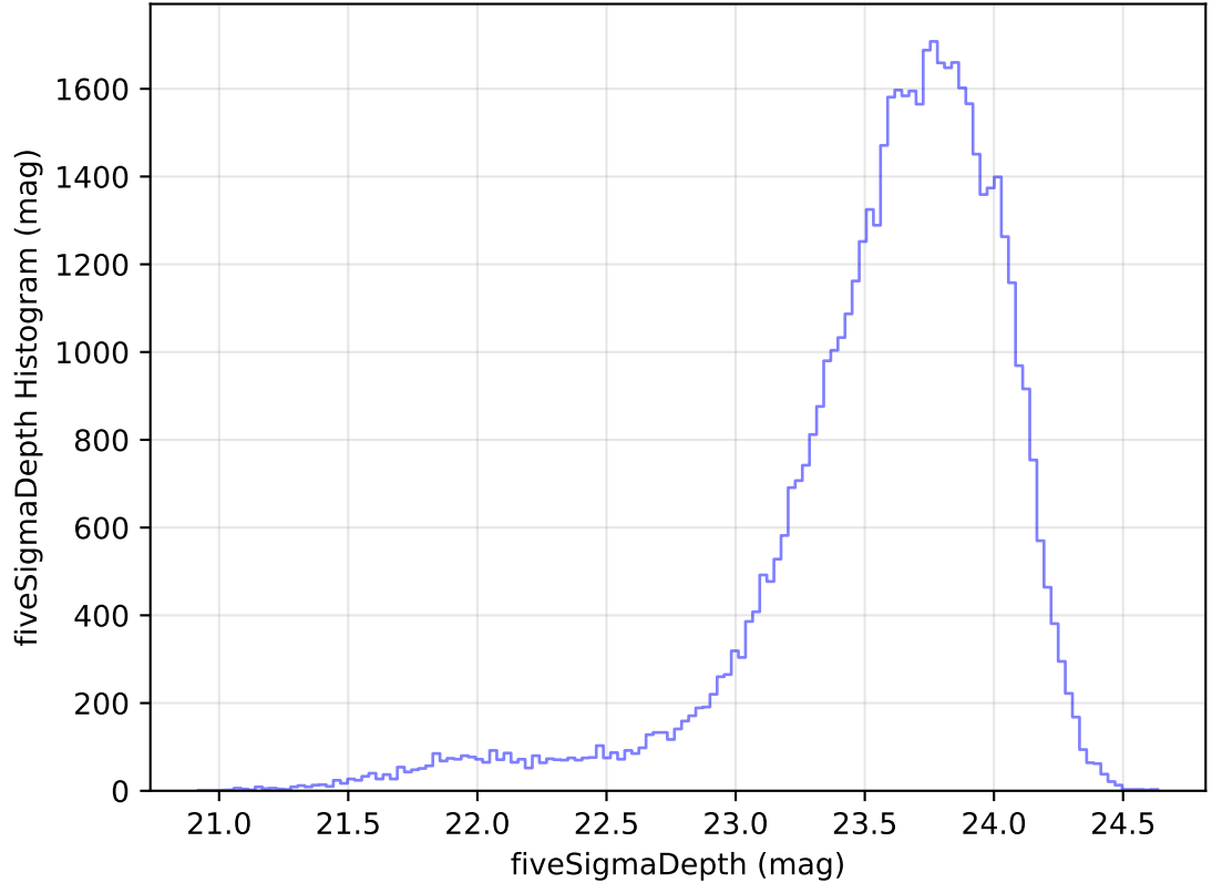
too_elab_heavy_r32_d2_ugrizy_v3.4_10yrs Yr 1 i band: fiveSigmaDepth Histogram
