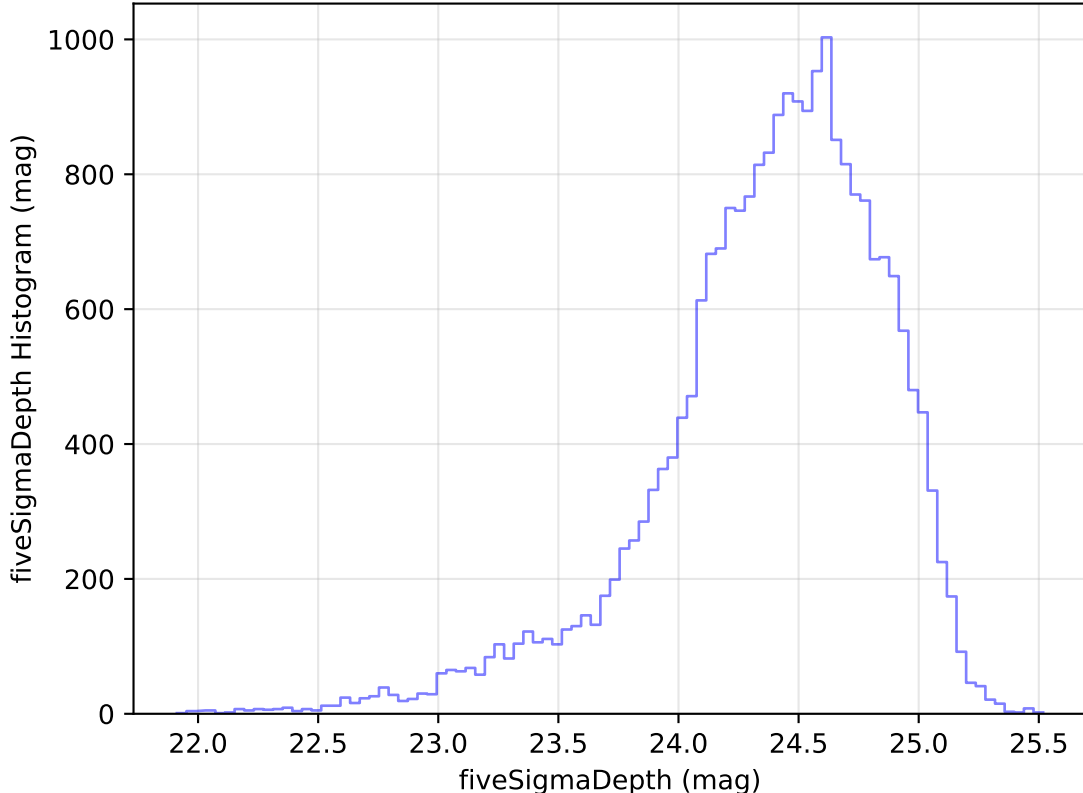
too_elab_heavy_r32_d2_ugrizy_v3.4_10yrs Yr 1 g band: fiveSigmaDepth Histogram
