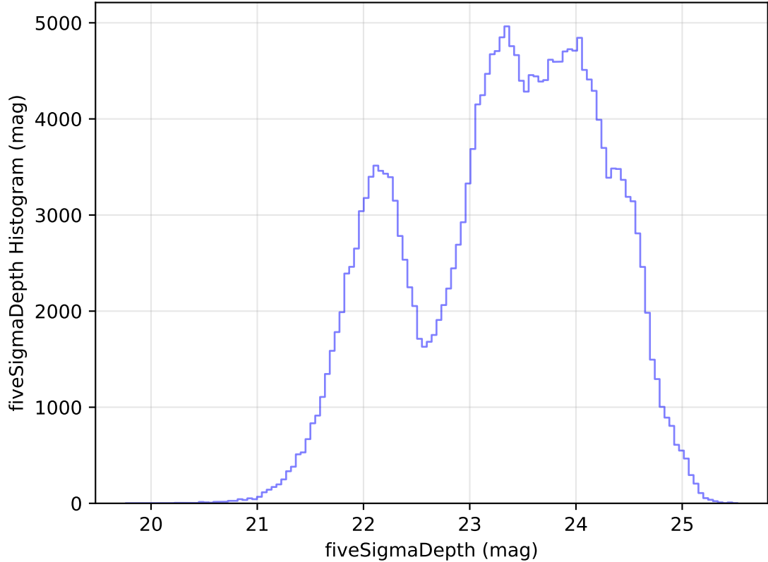
too_elab_heavy_r32_d2_ugrizy_v3.4_10yrs Yr 1 all bands: fiveSigmaDepth Histogram
