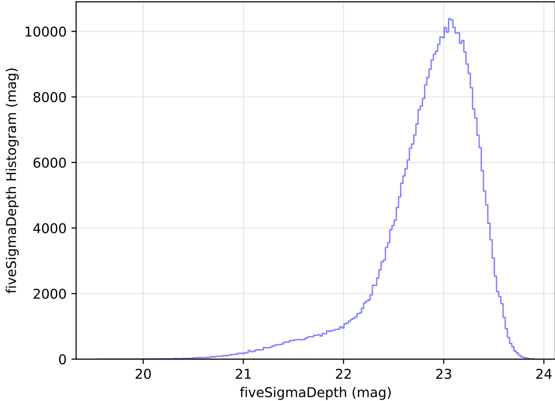
too_elab_heavy_r32_d2_ugrizy_v3.4_10yrs WFD z band: fiveSigmaDepth Histogram
