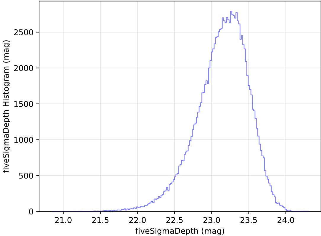
too_elab_heavy_r32_d2_ugrizy_v3.4_10yrs WFD u band: fiveSigmaDepth Histogram
