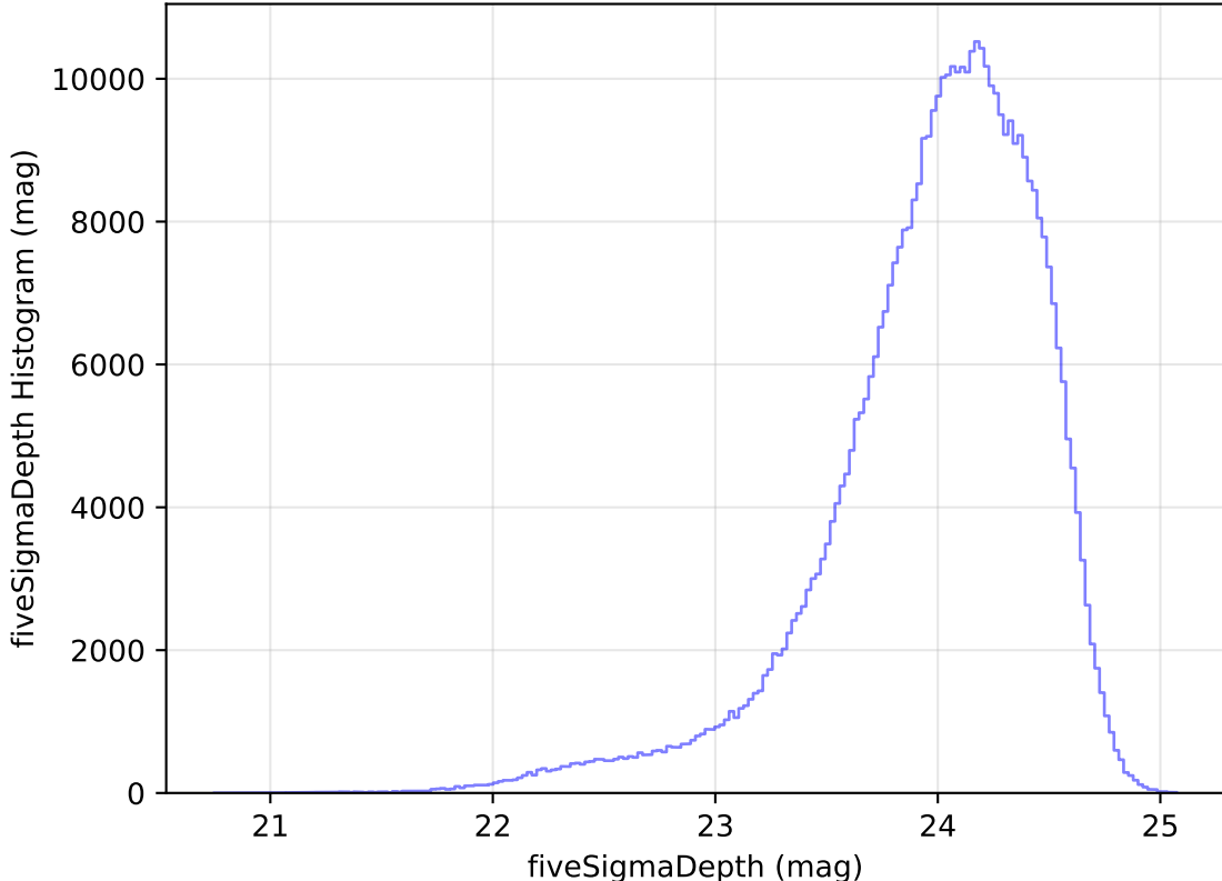
too_elab_heavy_r32_d2_ugrizy_v3.4_10yrs WFD r band: fiveSigmaDepth Histogram
