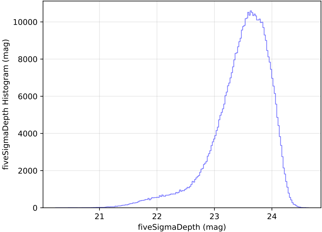
too_elab_heavy_r32_d2_ugrizy_v3.4_10yrs WFD i band: fiveSigmaDepth Histogram
