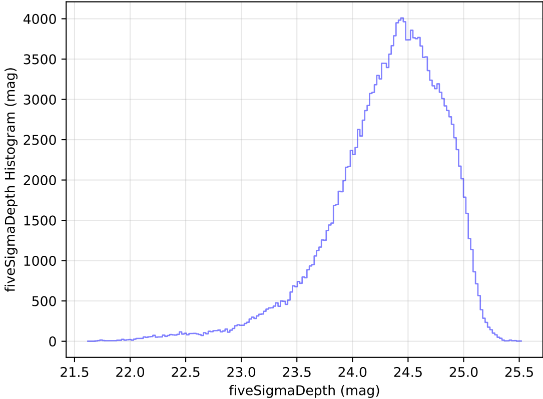
too_elab_heavy_r32_d2_ugrizy_v3.4_10yrs WFD g band: fiveSigmaDepth Histogram
