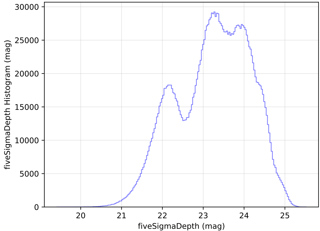
too_elab_heavy_r32_d2_ugrizy_v3.4_10yrs WFD all bands: fiveSigmaDepth Histogram
