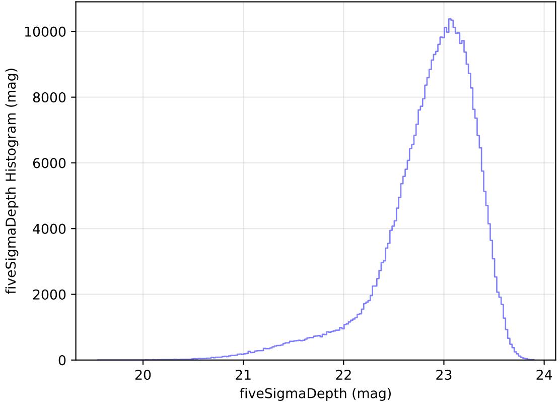
too_elab_heavy_r32_d2_ugrizy_v3.4_10yrs All sky z band: fiveSigmaDepth Histogram
