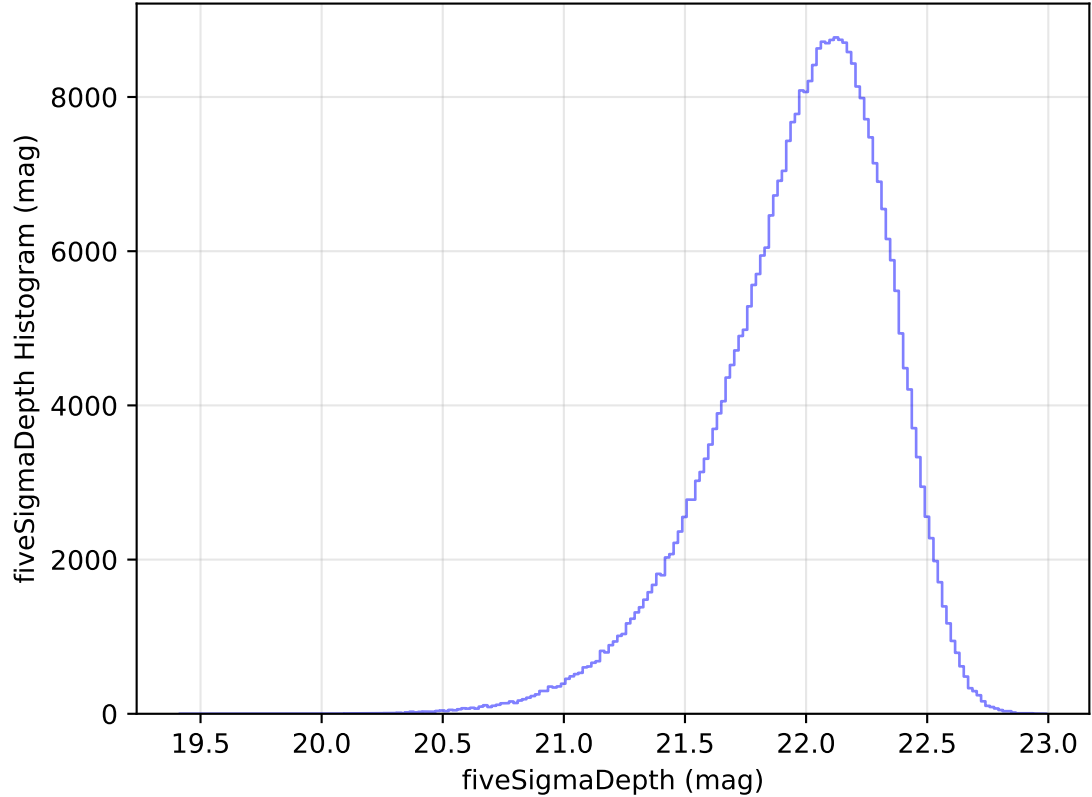
too_elab_heavy_r32_d2_ugrizy_v3.4_10yrs All sky y band: fiveSigmaDepth Histogram
