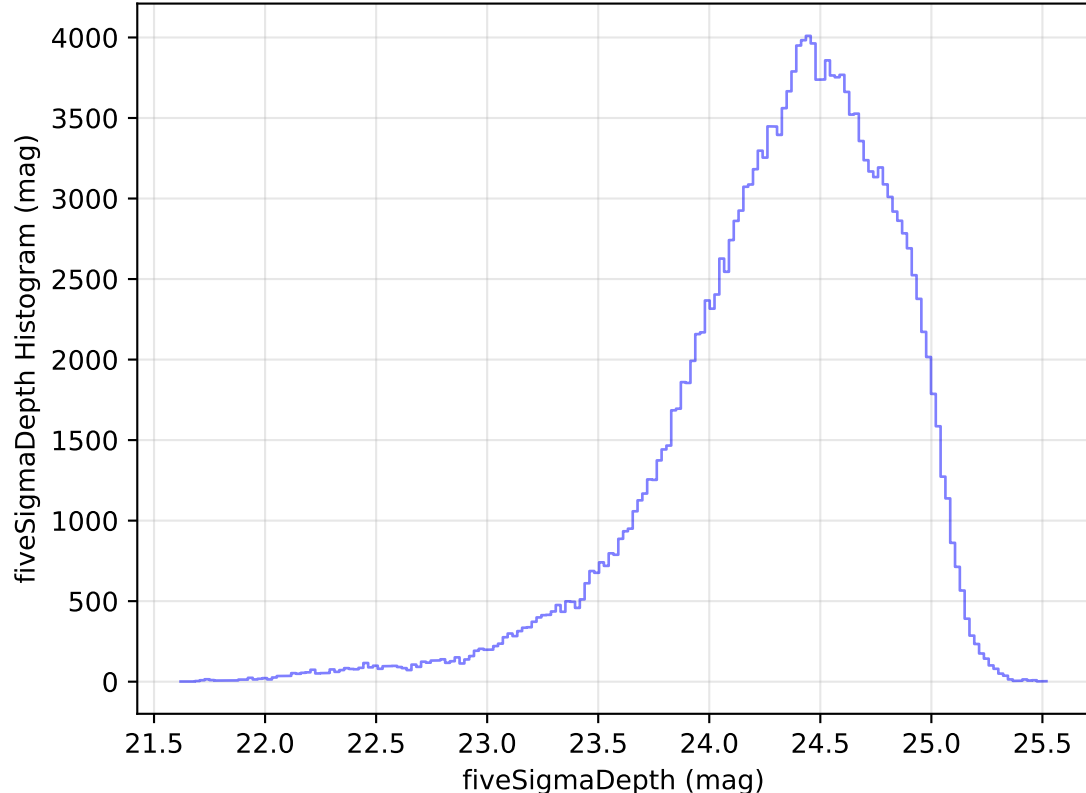
too_elab_heavy_r32_d2_ugrizy_v3.4_10yrs All sky g band: fiveSigmaDepth Histogram
