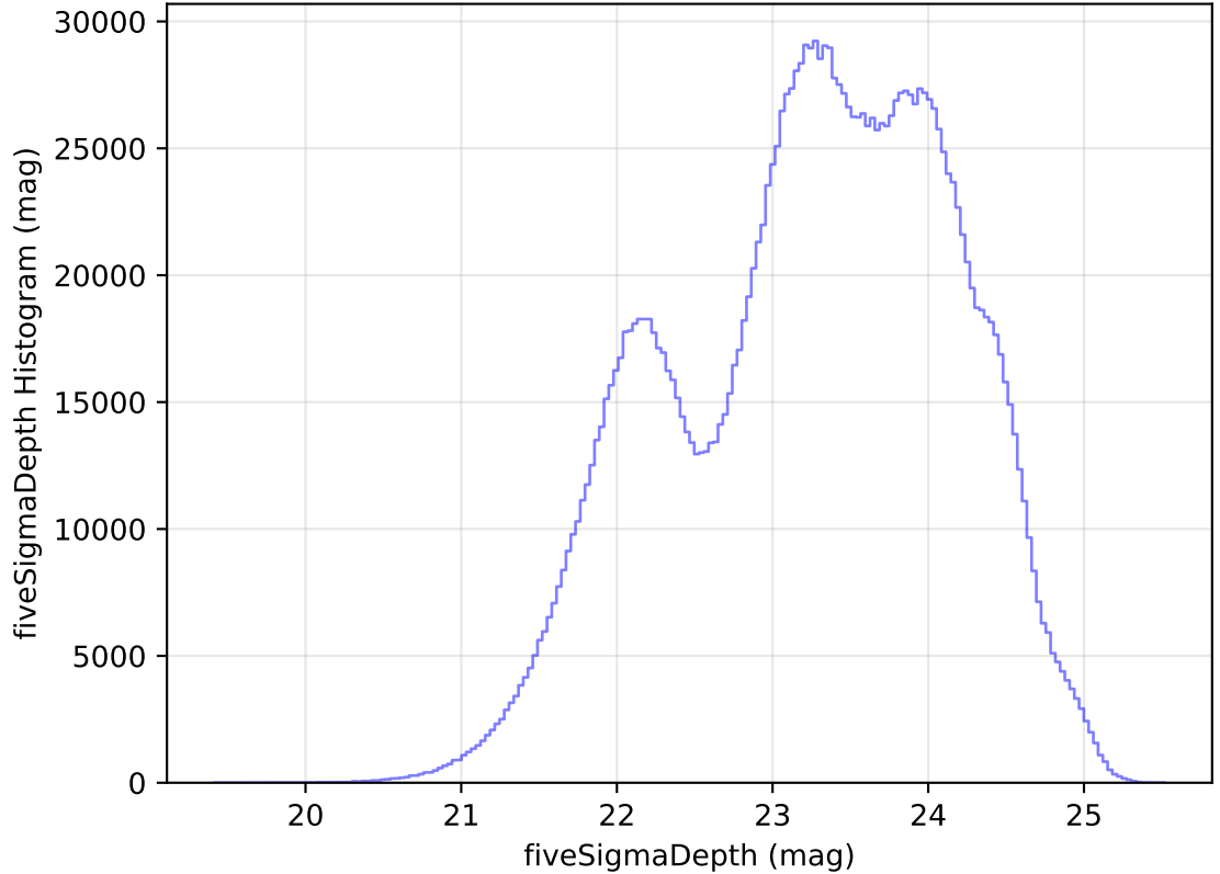
too_elab_heavy_r32_d2_ugrizy_v3.4_10yrs All sky all bands: fiveSigmaDepth Histogram
