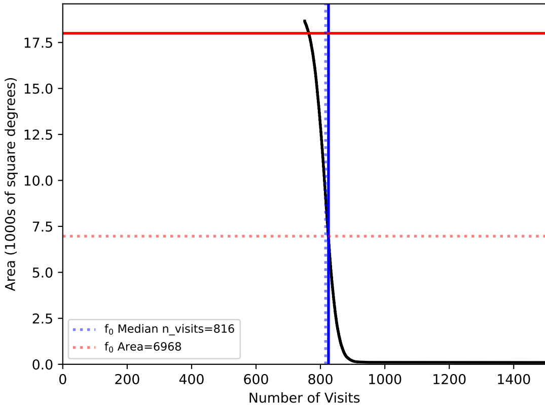
too_elab_heavy_r32_d2_ugrizy_v3.4_10yrs WFD: f0
