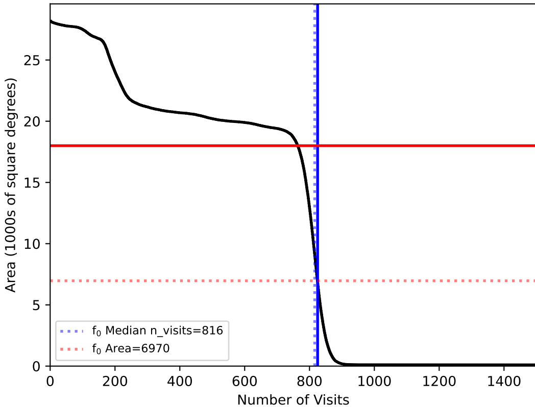
too_elab_heavy_r32_d2_ugrizy_v3.4_10yrs All sky: f0
