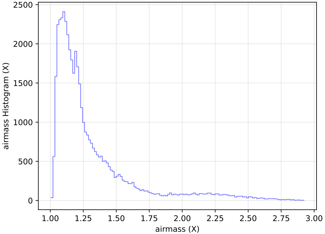
too_elab_heavy_r32_d2_ugrizy_v3.4_10yrs Yr 1 z band: airmass Histogram
