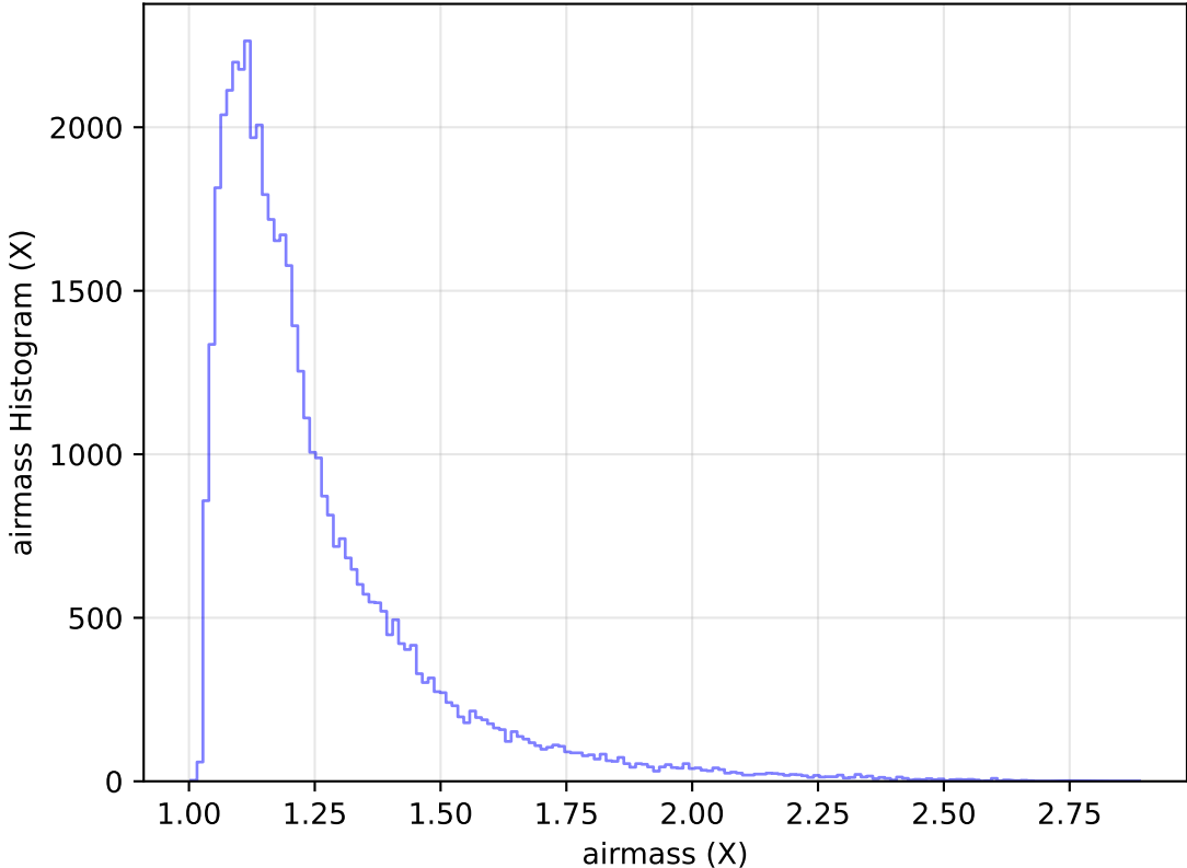
too_elab_heavy_r32_d2_ugrizy_v3.4_10yrs Yr 1 y band: airmass Histogram
