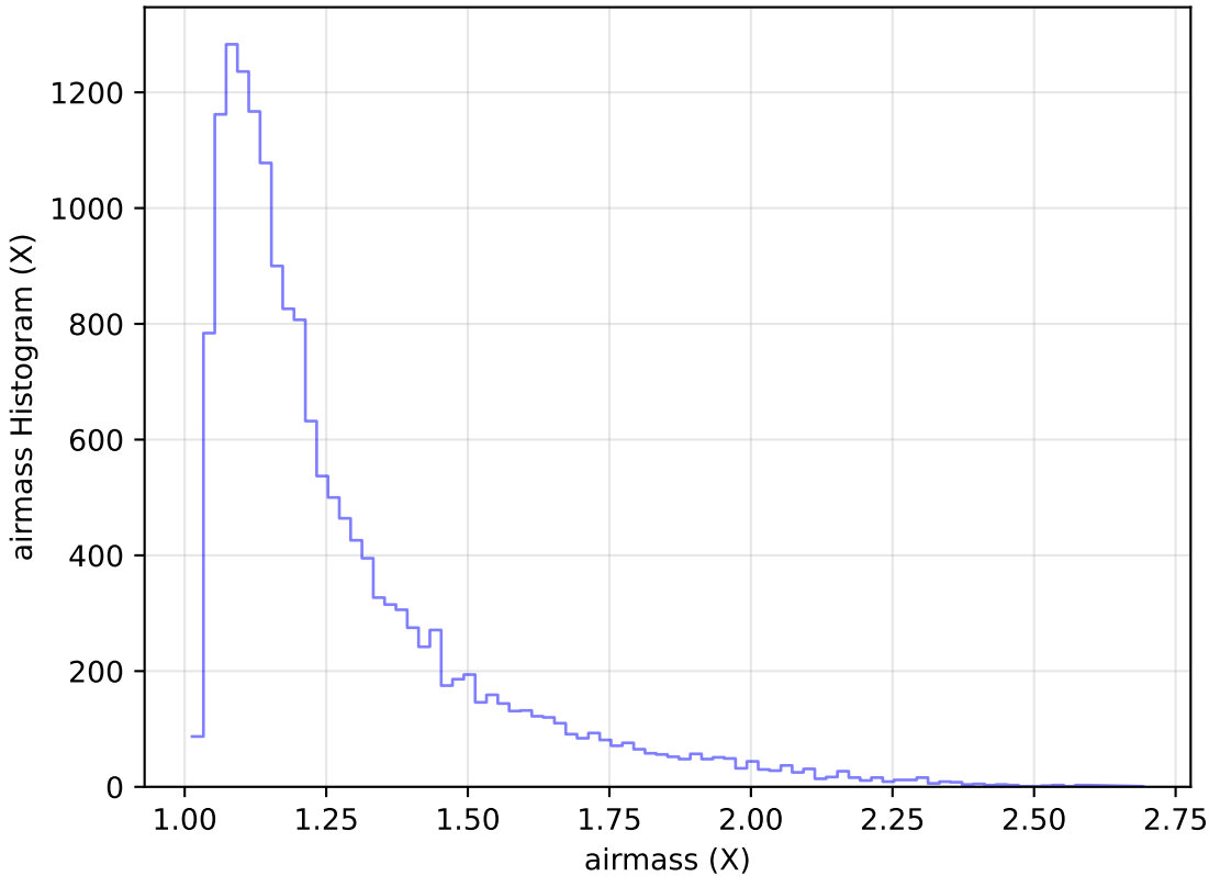
too_elab_heavy_r32_d2_ugrizy_v3.4_10yrs Yr 1 u band: airmass Histogram
