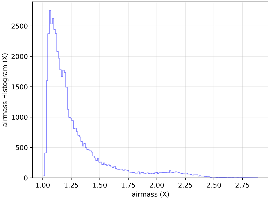
too_elab_heavy_r32_d2_ugrizy_v3.4_10yrs Yr 1 r band: airmass Histogram
