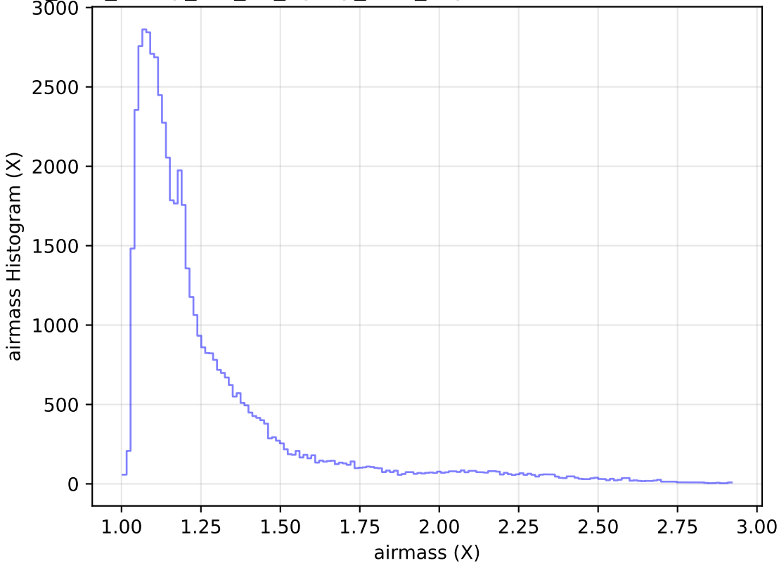
too_elab_heavy_r32_d2_ugrizy_v3.4_10yrs Yr 1 i band: airmass Histogram
