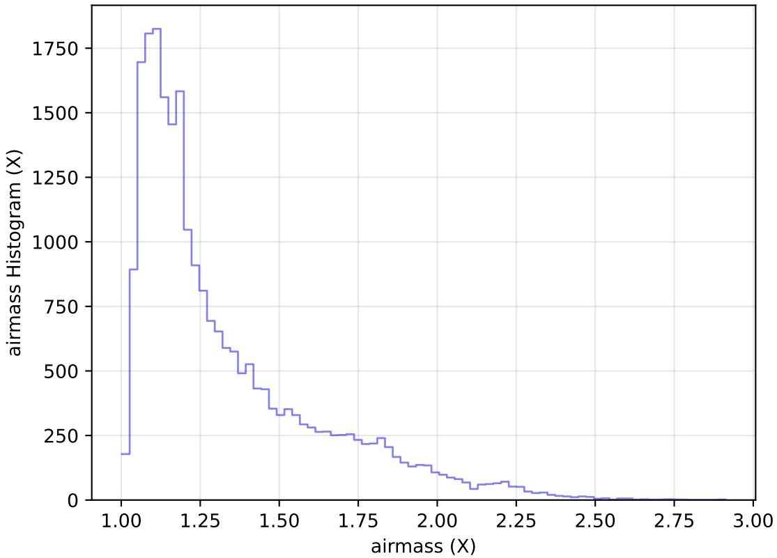
too_elab_heavy_r32_d2_ugrizy_v3.4_10yrs Yr 1 g band: airmass Histogram
