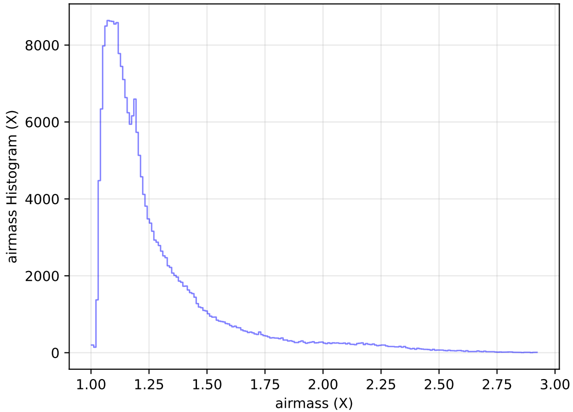
too_elab_heavy_r32_d2_ugrizy_v3.4_10yrs Yr 1 all bands: airmass Histogram
