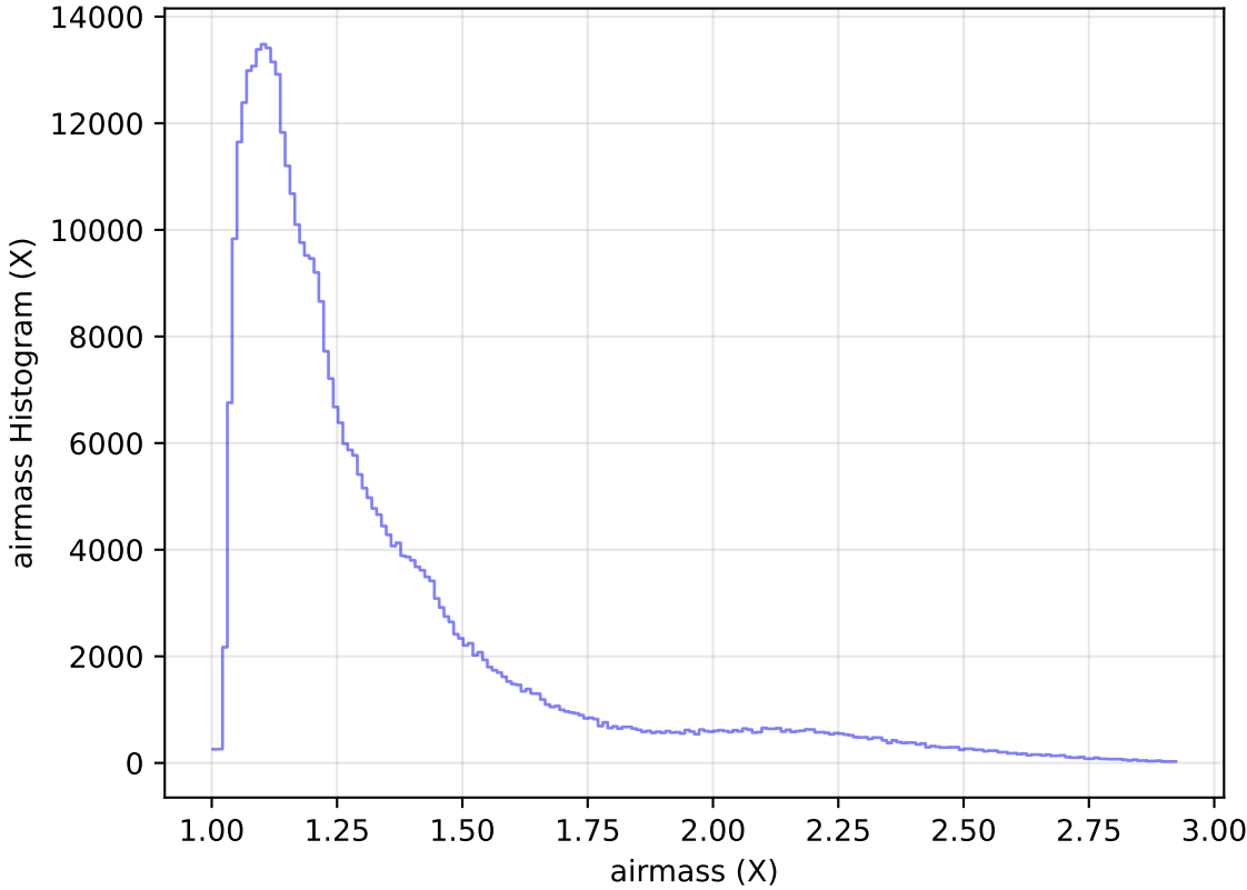
too_elab_heavy_r32_d2_ugrizy_v3.4_10yrs WFD z band: airmass Histogram
