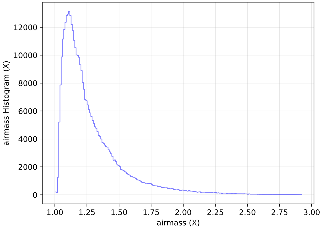
too_elab_heavy_r32_d2_ugrizy_v3.4_10yrs WFD y band: airmass Histogram
