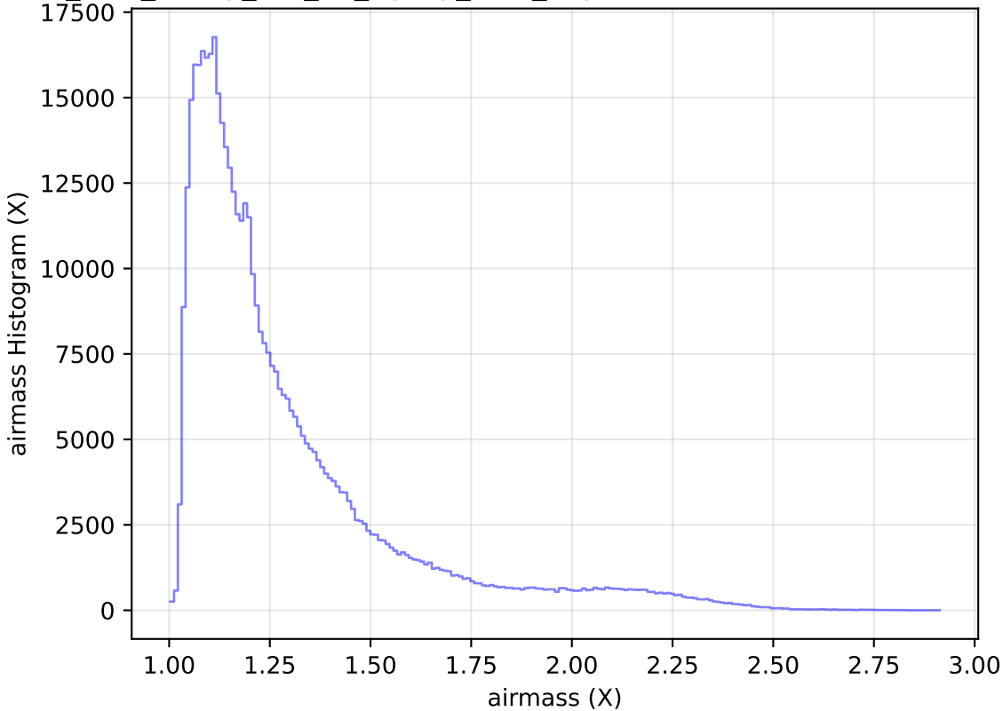
too_elab_heavy_r32_d2_ugrizy_v3.4_10yrs WFD r band: airmass Histogram
