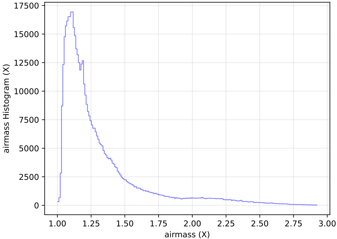
too_elab_heavy_r32_d2_ugrizy_v3.4_10yrs WFD i band: airmass Histogram
