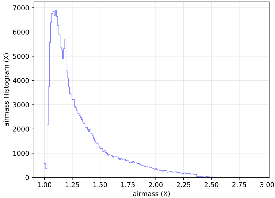
too_elab_heavy_r32_d2_ugrizy_v3.4_10yrs WFD g band: airmass Histogram
