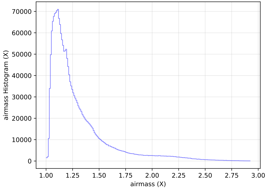
too_elab_heavy_r32_d2_ugrizy_v3.4_10yrs WFD all bands: airmass Histogram
