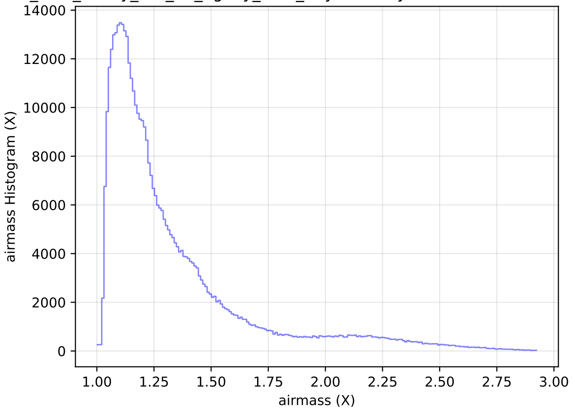
too_elab_heavy_r32_d2_ugrizy_v3.4_10yrs All sky z band: airmass Histogram
