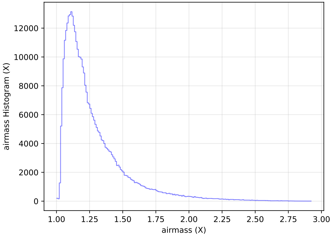
too_elab_heavy_r32_d2_ugrizy_v3.4_10yrs All sky y band: airmass Histogram
