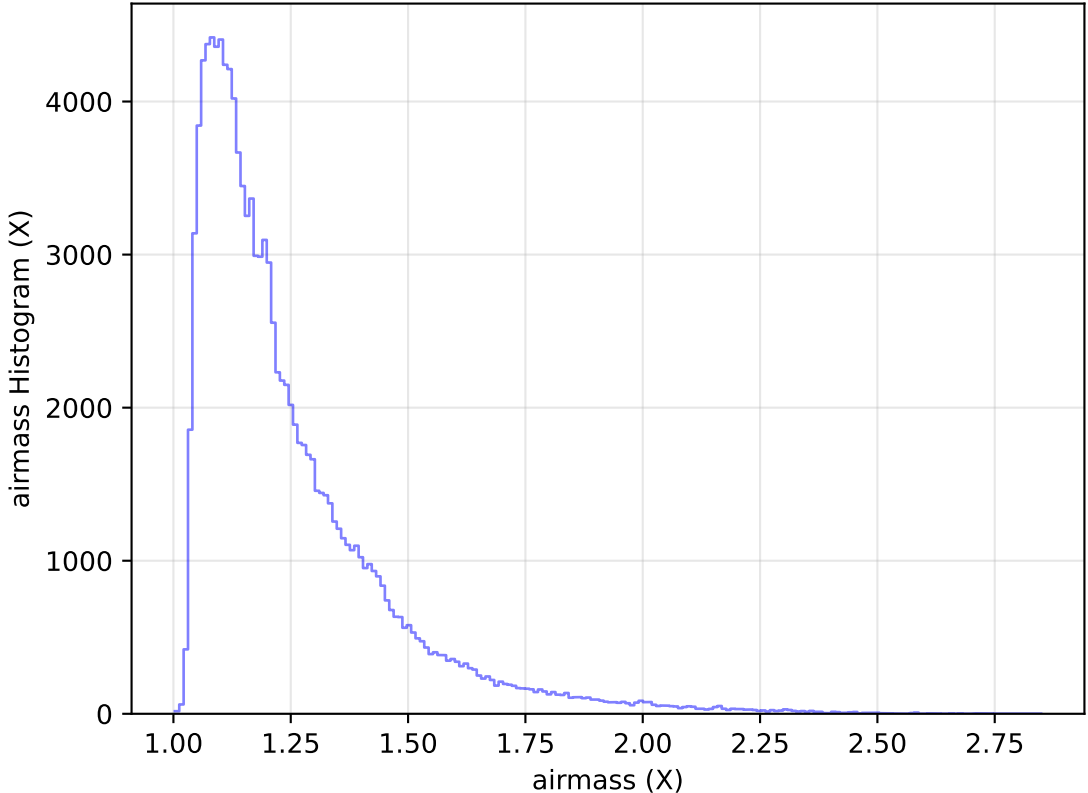
too_elab_heavy_r32_d2_ugrizy_v3.4_10yrs All sky u band: airmass Histogram
