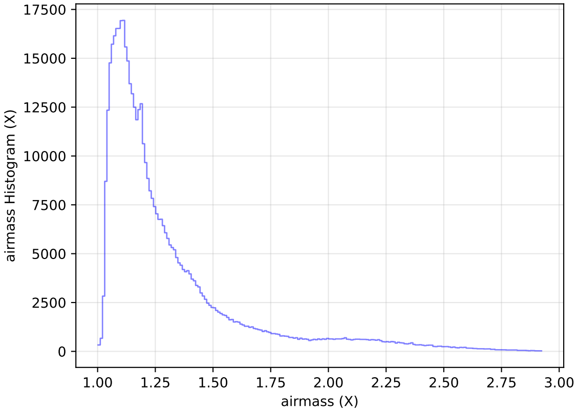
too_elab_heavy_r32_d2_ugrizy_v3.4_10yrs All sky i band: airmass Histogram
