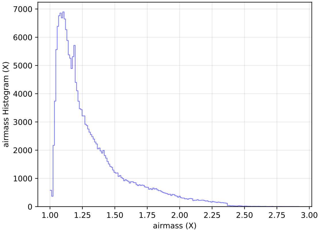
too_elab_heavy_r32_d2_ugrizy_v3.4_10yrs All sky g band: airmass Histogram
