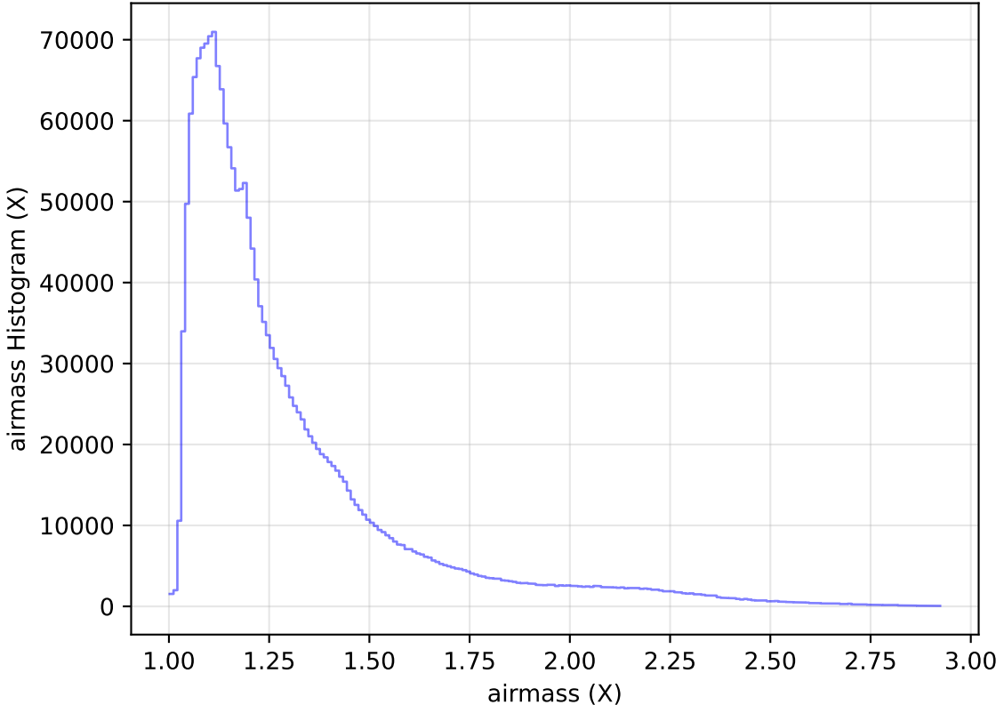
too_elab_heavy_r32_d2_ugrizy_v3.4_10yrs All sky all bands: airmass Histogram
