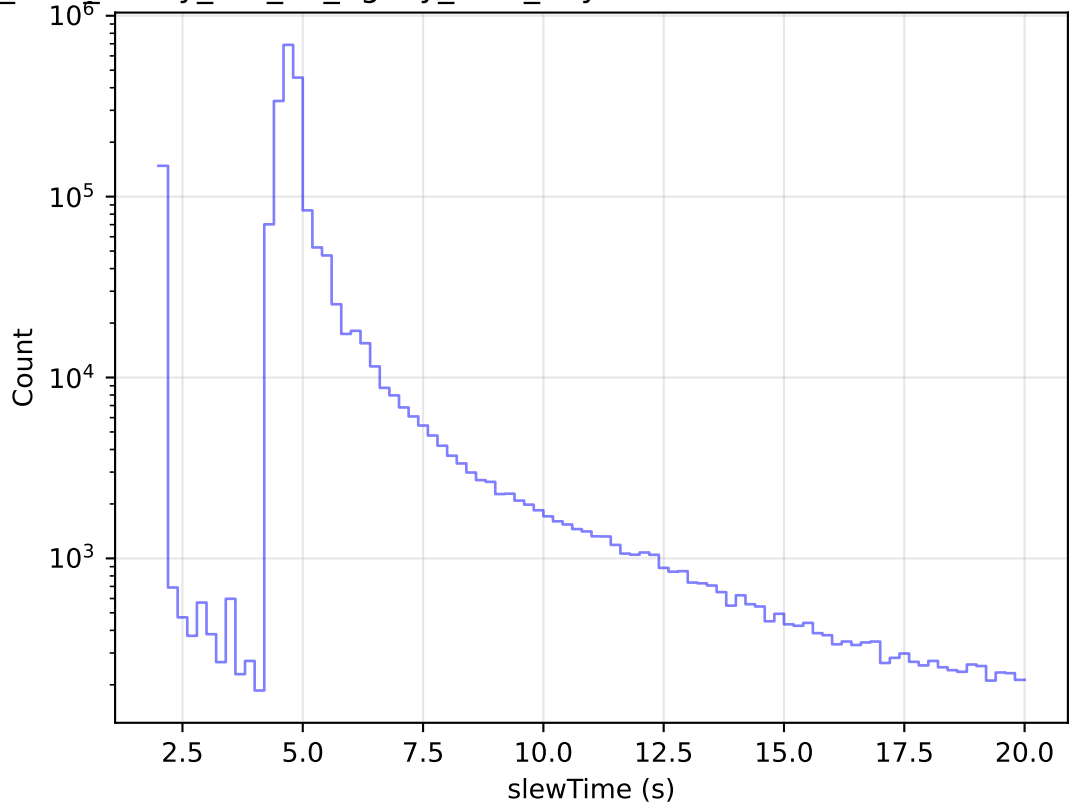
too_elab_heavy_r32_d2_ugrizy_v3.4_10yrs All visits: Zoom Slew Time Histogram
