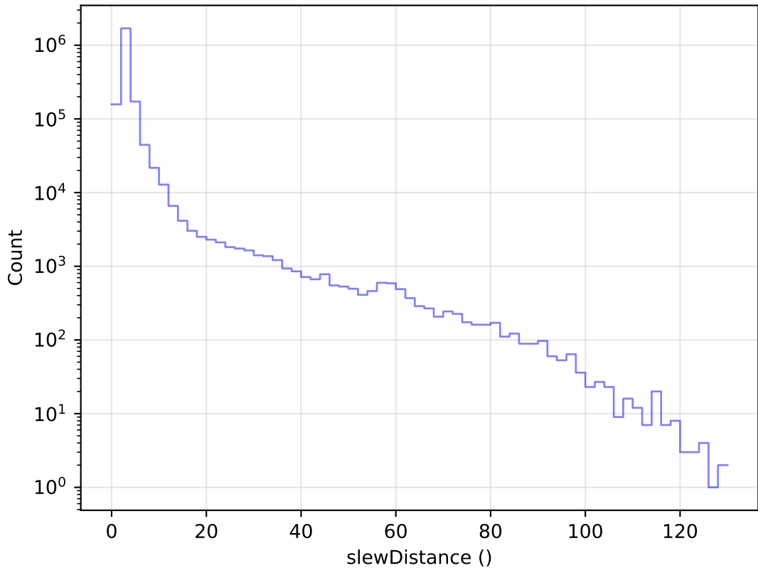
too_elab_heavy_r32_d2_ugrizy_v3.4_10yrs All visits: Slew Distance Histogram
