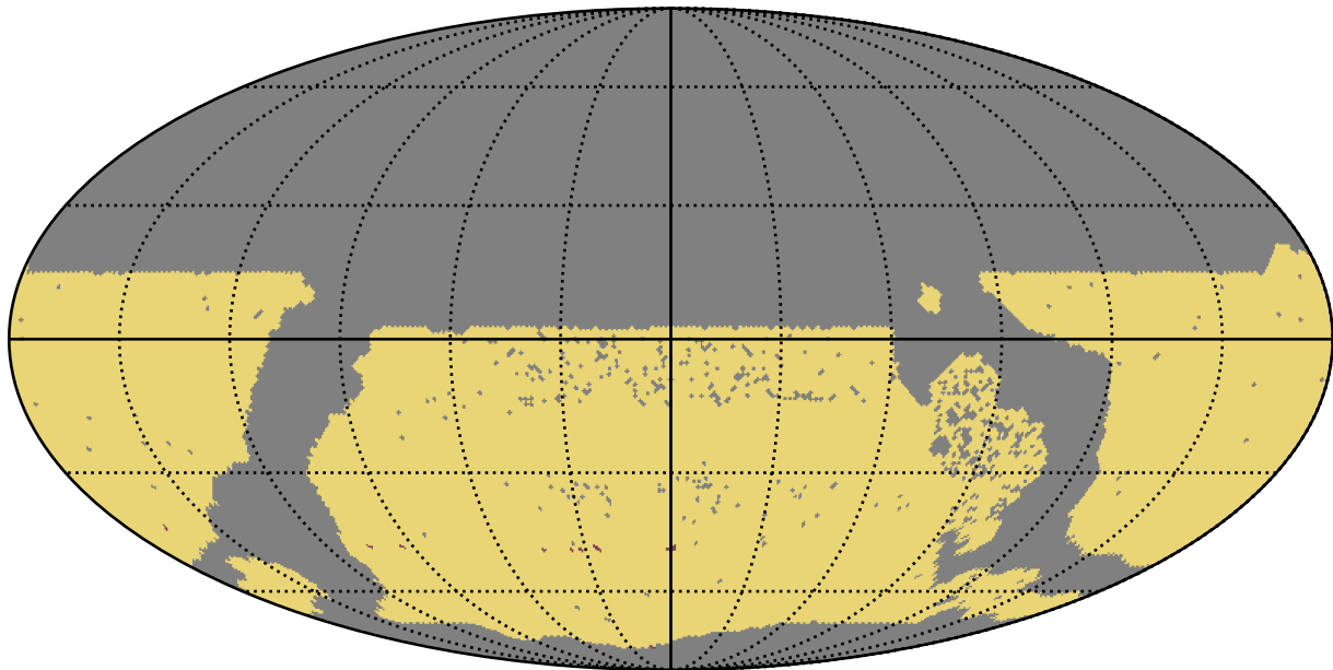
too_elab_heavy_r32_d2_ugrizy_v3.4_10yrs WFD: RapidRevisits
