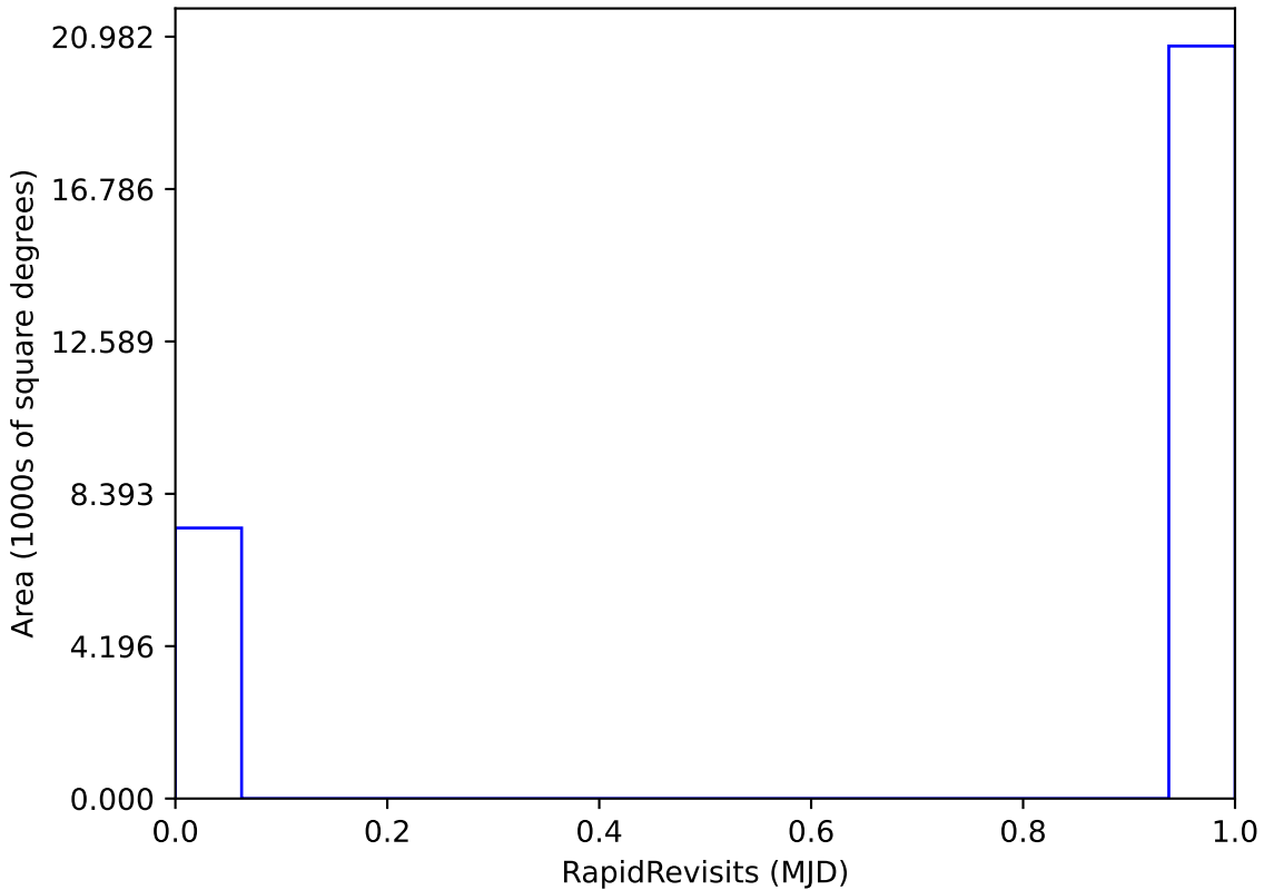
too_elab_heavy_r32_d2_ugrizy_v3.4_10yrs All sky: RapidRevisits
