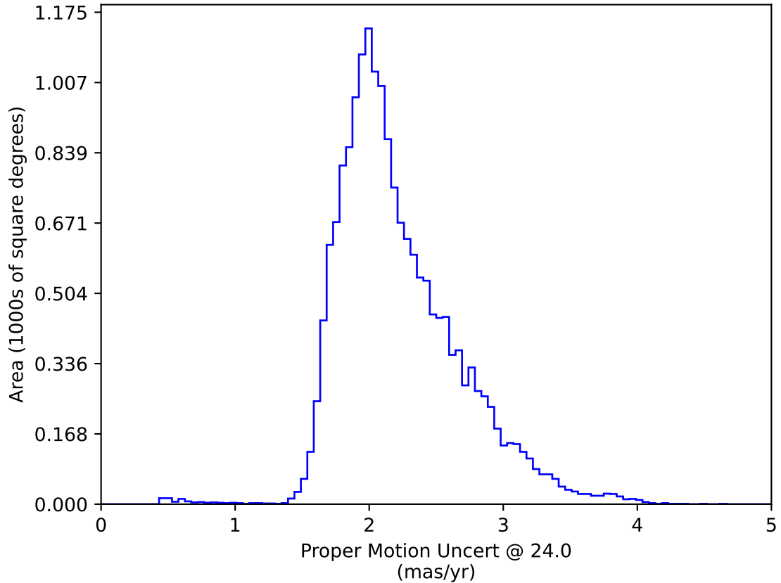
too_elab_heavy_r32_d2_ugrizy_v3.4_10yrs WFD: Proper Motion Uncert @ 24.0
