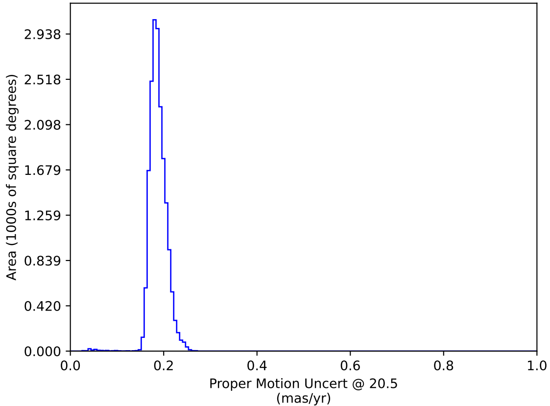
too_elab_heavy_r32_d2_ugrizy_v3.4_10yrs WFD: Proper Motion Uncert @ 20.5
