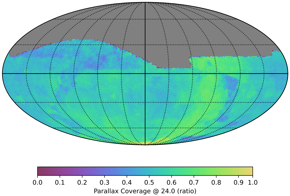
too_elab_heavy_r32_d2_ugrizy_v3.4_10yrs All sky: Parallax Coverage @ 24.0
