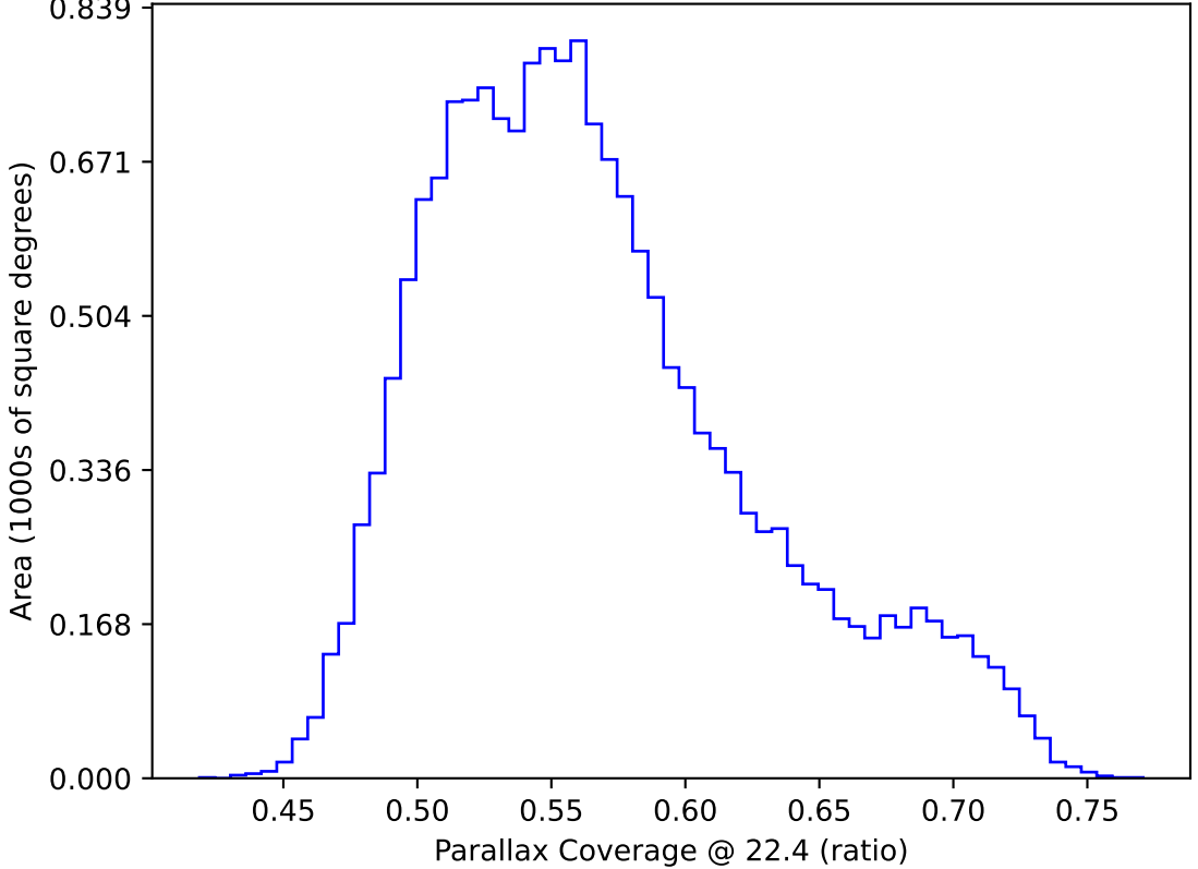
too_elab_heavy_r32_d2_ugrizy_v3.4_10yrs WFD: Parallax Coverage @ 22.4
