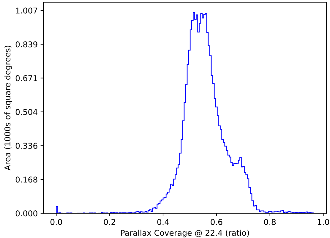
too_elab_heavy_r32_d2_ugrizy_v3.4_10yrs All sky: Parallax Coverage @ 22.4
