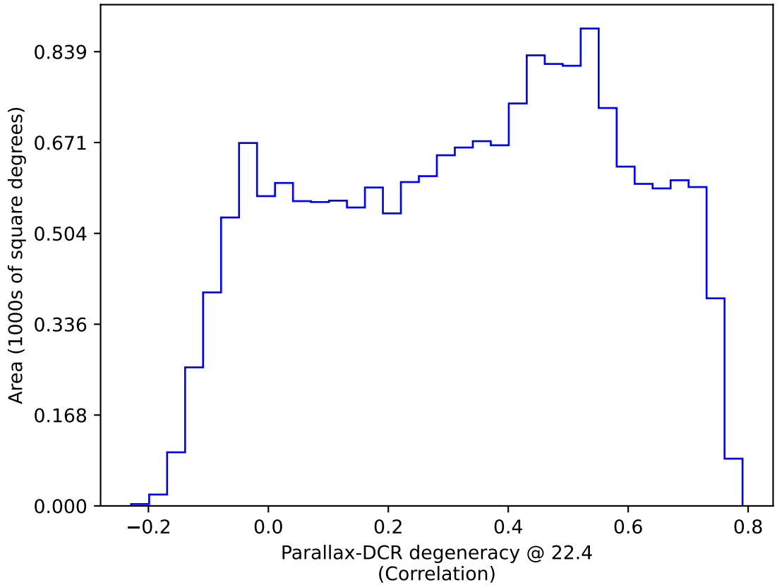
too_elab_heavy_r32_d2_ugrizy_v3.4_10yrs WFD: Parallax-DCR degeneracy @ 22.4
