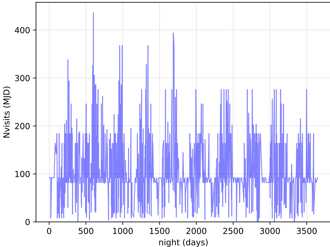
too_elab_heavy_r32_d2_ugrizy_v3.4_10yrs DDF: Nvisits
