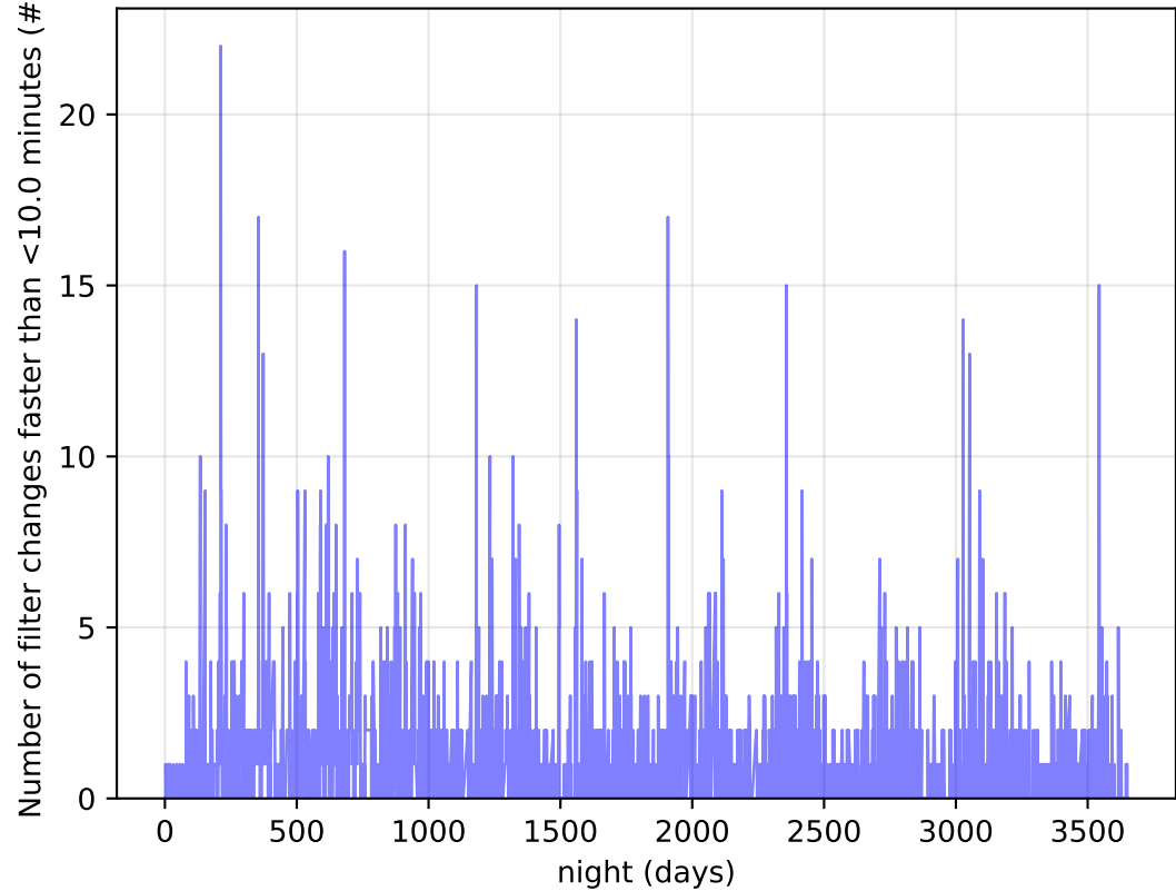
too_elab_heavy_r32_d2_ugrizy_v3.4_10yrs Per Night: Number of filter changes faster than <10.0 minutes
